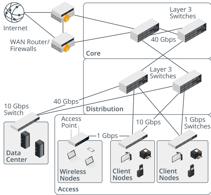
Network infrastructure diagram. (Images © 123RF.com)
